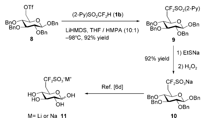
Scheme 3. Synthesis of fluorinated β-pyranoside sulfonate 11 . Bn = benzyl.
